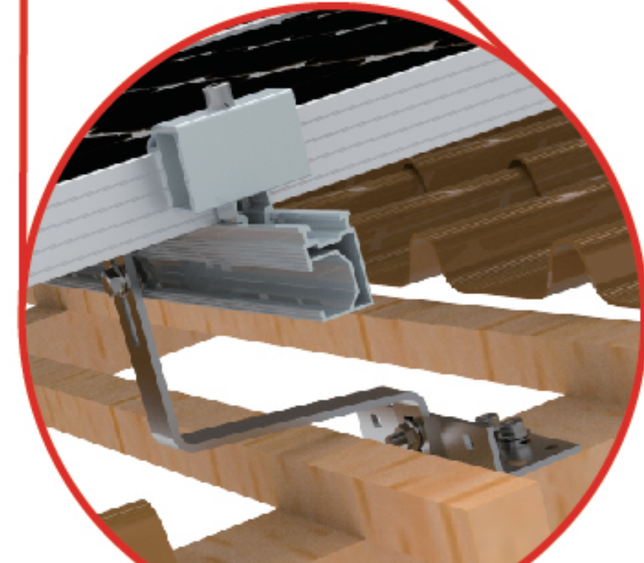
Detail in Side View
